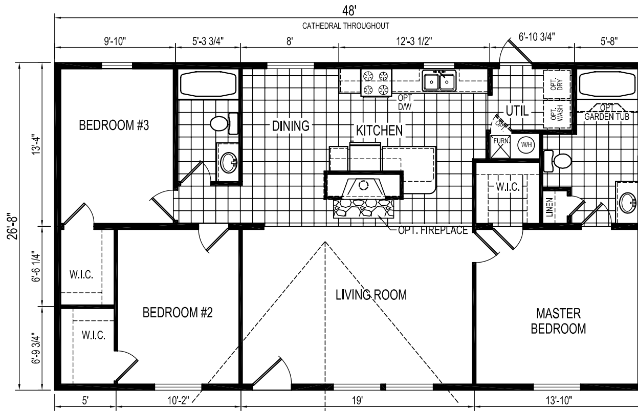
MODEL 122-A-136 3 BEDROOM, 2 BATH NOMINAL SIZE: 28' x 52' TOTAL AREA: 1280 SQ. FT.
