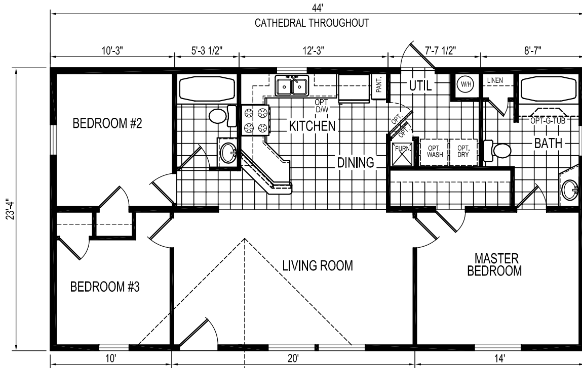
MODEL 122-A-262 3 BEDROOM, 2 BATH NOMINAL SIZE: 24' x 48' TOTAL AREA: 1,026 SQ. FT.
