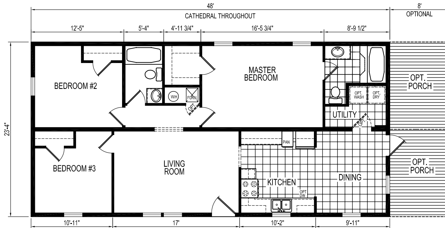
MODEL 122-A-288 3 BEDROOM, 2 BATH NOMINAL SIZE: 24' x 52' TOTAL AREA: 1120 SQ. FT.
