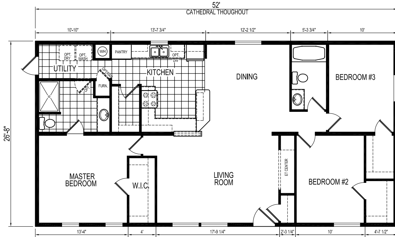
MODEL 122-A-509 3 BEDROOM, 2 BATH NOMINAL SIZE: 28' x 56' TOTAL AREA: 1,387 SQ. FT.
