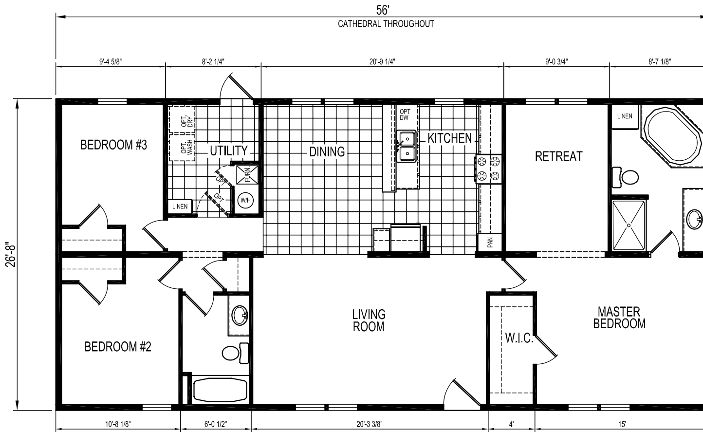
MODEL 122-A-515 3 BEDROOM, 2 BATH NOMINAL SIZE: 28' x 60' TOTAL AREA: 1,493 SQ. FT.
