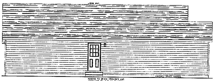
LEFT ELEVATION
